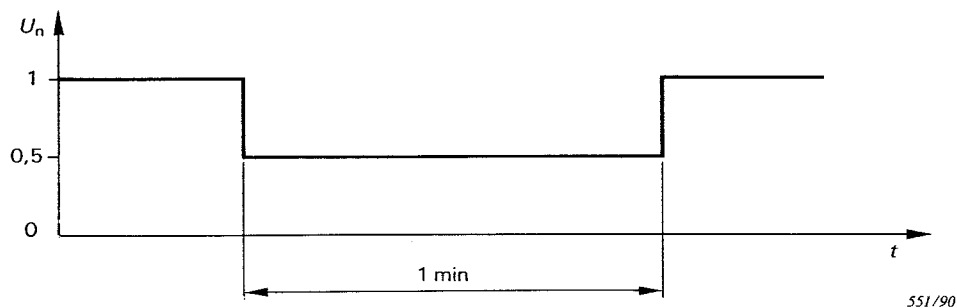
Figure B.3 – Creux de tension \Delta U = 50 \%
